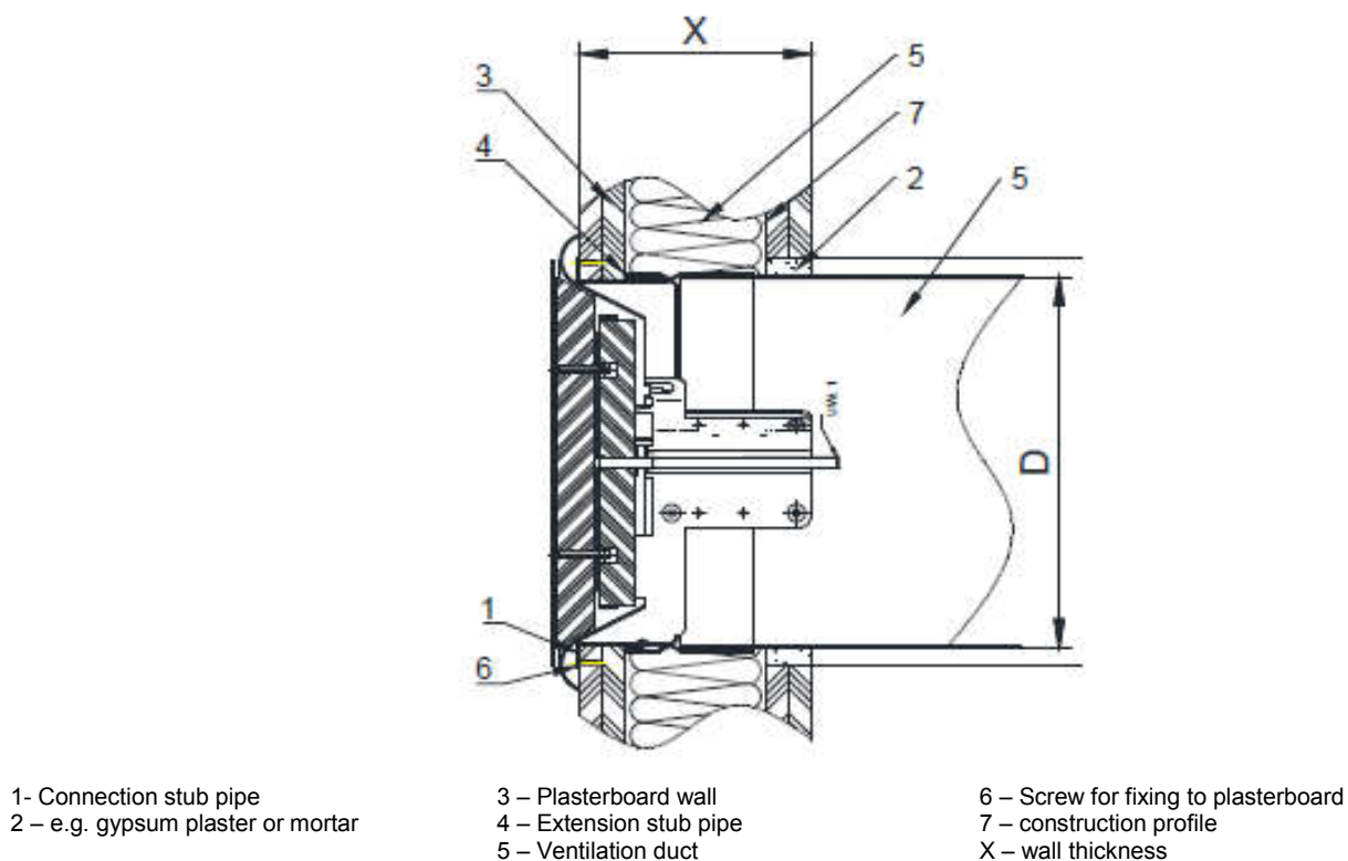
Figure 10. Sample installation of the mcr ZIPP valve in a plasterboard wall.
